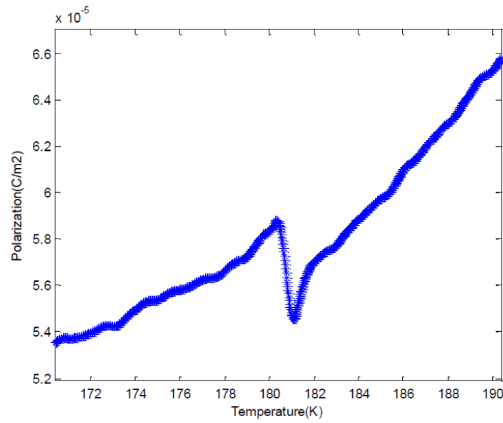
Figure 19: Polarization of pyroelectric current with negative poling electric field
