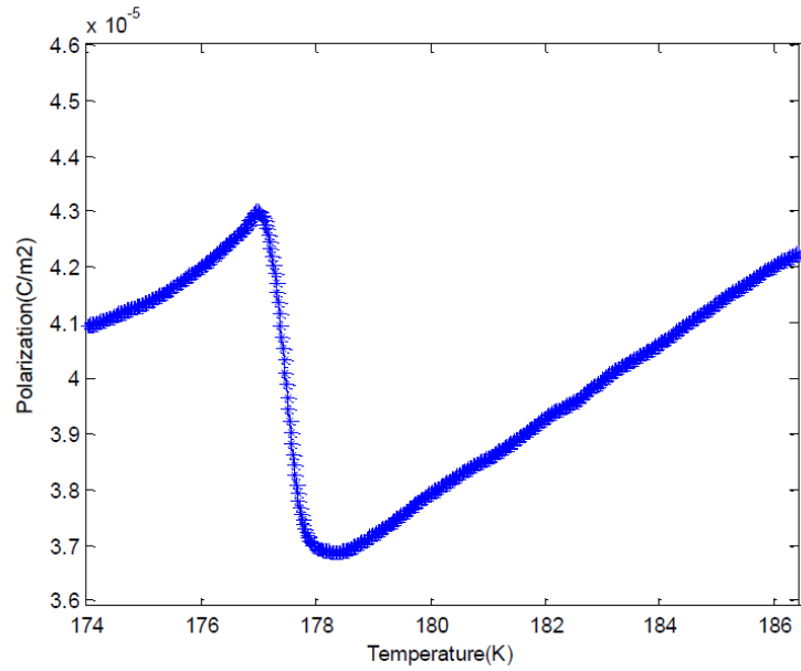
Figure 25: Polarization of pyroelectric current with negative poling electric field
