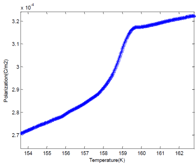
Figure 30: Polarization of pyroelectric current with positive poling electric field
