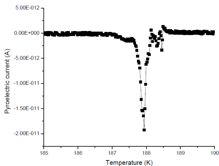
Figure 47: Pyroelectric current after poling with negative electric field -300 V
